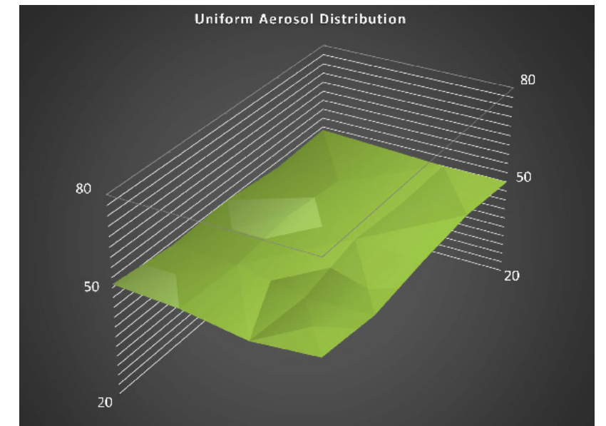
As can be seen in the aerosol distribution profile of the Pharmaseal FFU, our system deviates less than 7% from the target aerosol concentration of 50 µg/l. The industry standard is 20% relative aerosol deviation with <50% local aerosol deviance. Sample location and test protocol along with results for various FFU configurations are available upon request.
